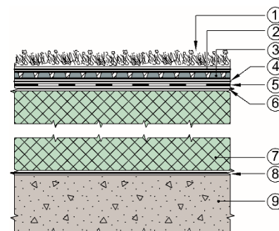
Fig. 1 Protan SE roofing membranes, mechanically fastened at the edge
