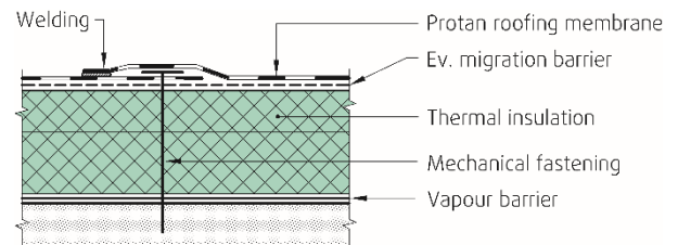
Fig. 1 Protan SE roofing membranes, mechanically fastened at the edge
